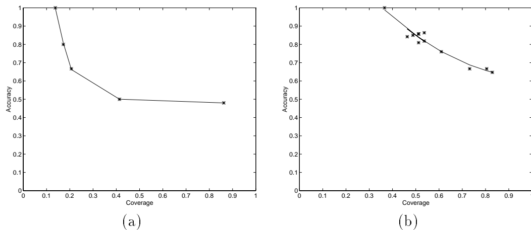
Fig. 6. Sample matching results: the graphs shows accuracy versus coverage for a range of reliability threshold values. A low threshold implies high coverage and low accuracy, while a high threshold implies low coverage and high accuracy. (a) Results for a 60-second video sequence containing 29 vehicles detected at both cameras as well as over 40 entering and exiting vehicles. (b) Results for the same sequence with the tracks of entering and exiting vehicles removed, to simulate performance on freeway sections without onramps and offramps.
